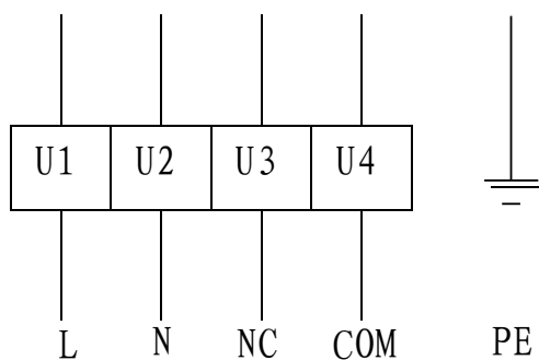
Power Line
